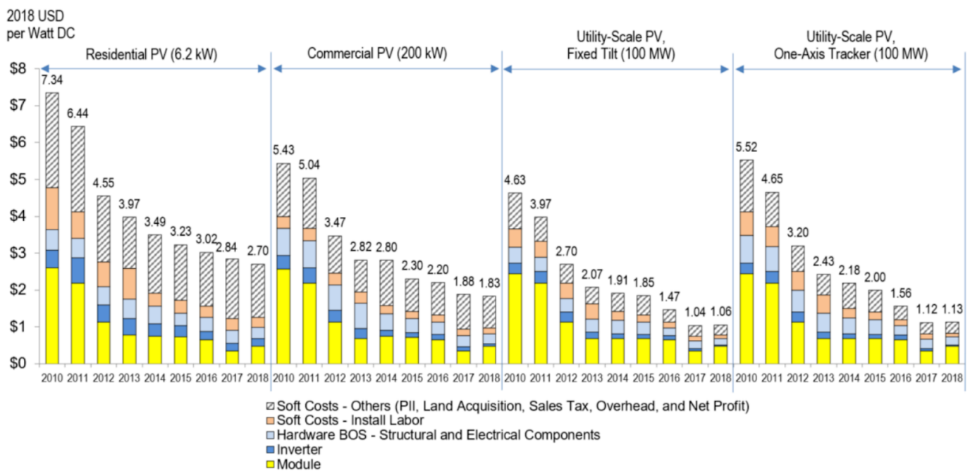
Fig. 27: PV system cost benchmark summary, 2010-2018 (Figure 2)
