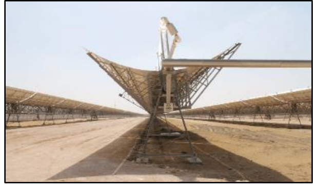
Fig.22: The Parabolic Trough is a long trough in the shape of a parabola with a reflective surface. Light converges on a point, generating heat. (Irena, 2015)
