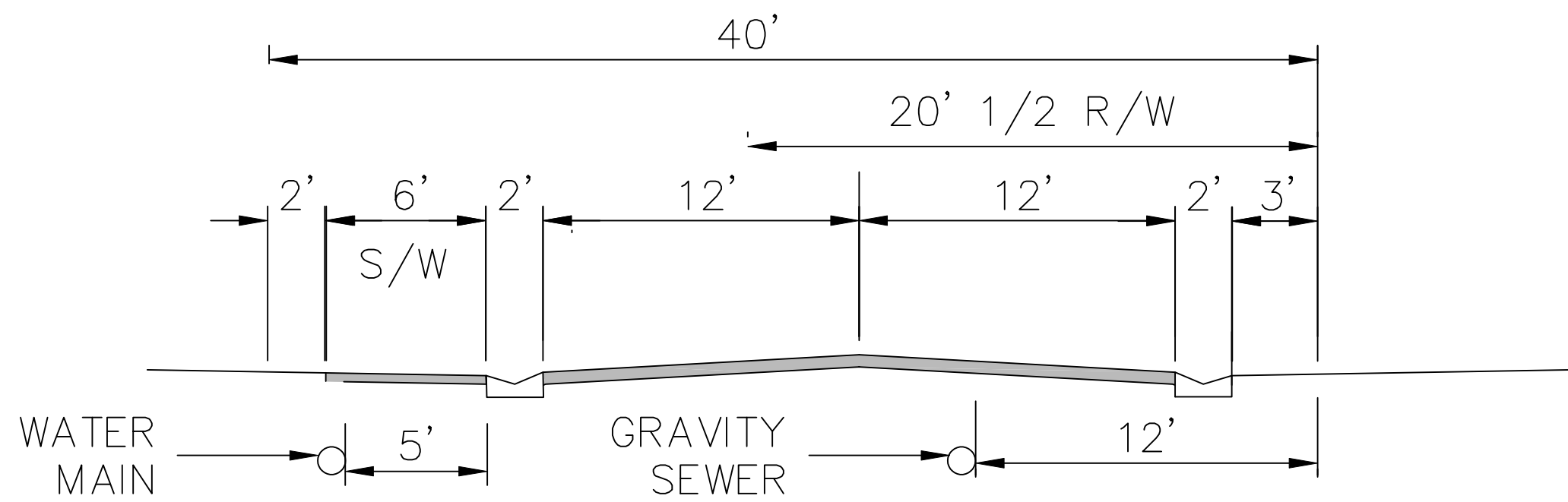
NOTE: UTILITIES MAY SHIFT BASED UPON DRAINAGE PIPE LOCATION W/ RIGHT OF WAY TYPICAL ROAD SECTION NTS
